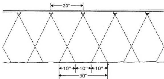
Figure 2.7.2. Fifty percent overlap.
